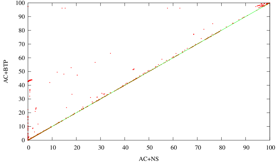
Figure 13: Percentage of values removed by AC and neighbourhood substitution (AC+NS) vs percentage of values removed by AC and BTP-merging (AC+BTP) for each considered instance.
